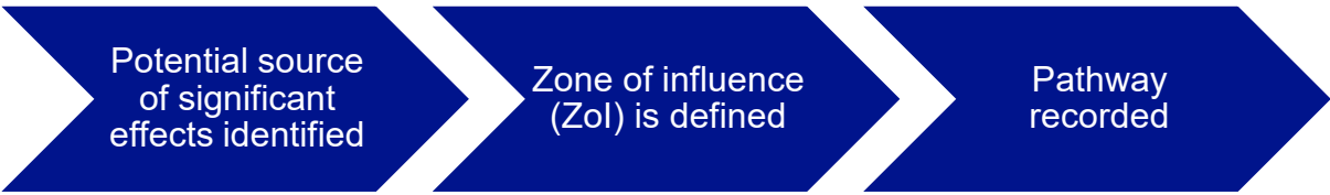
Image 8.1 Source-Pathway-Receptor Approach
